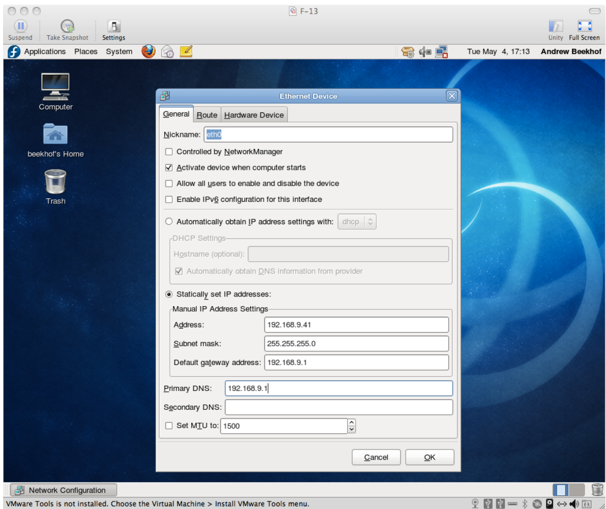
Figure 2.15. Fedora Installation - Specify Network Preferences
