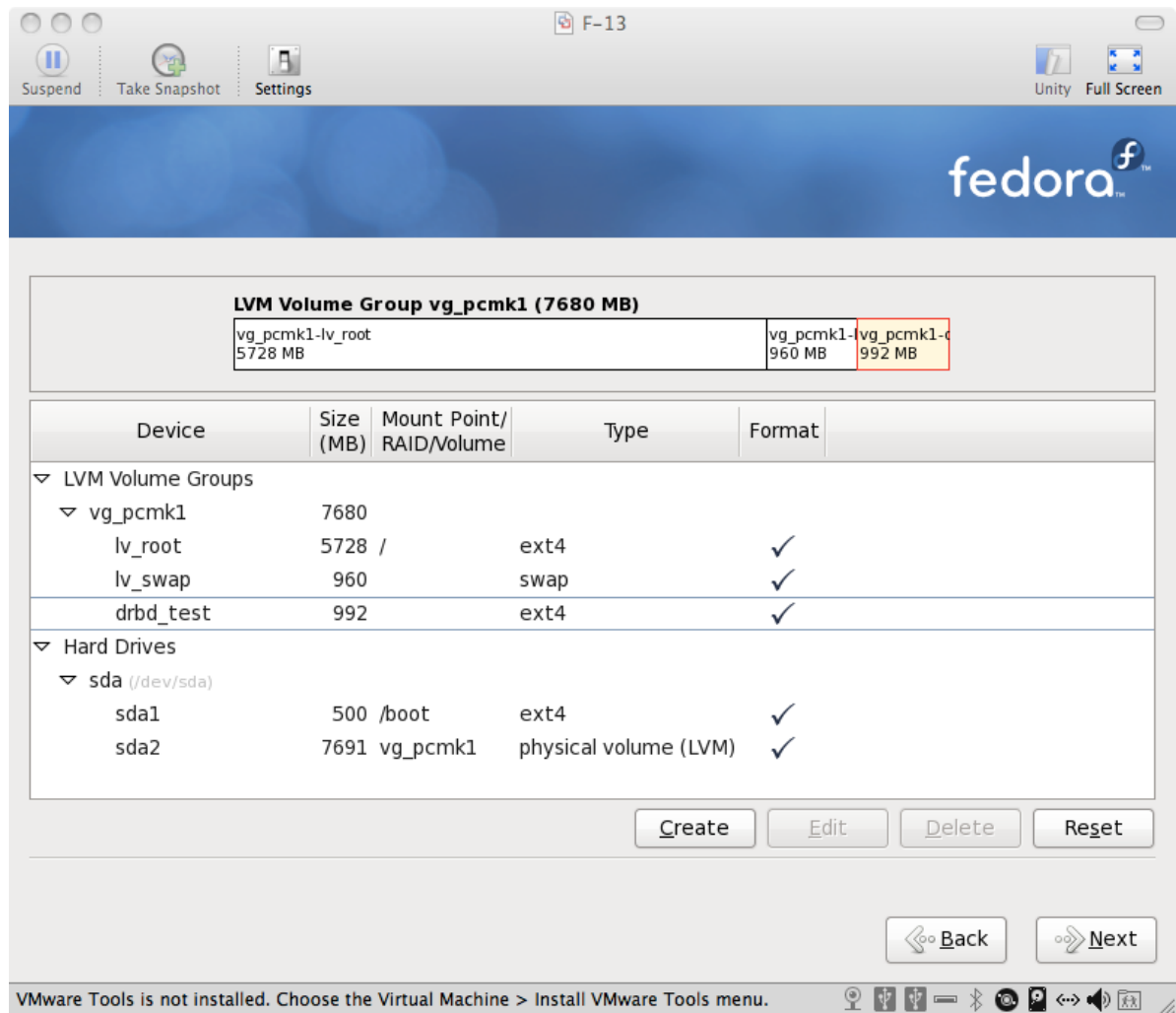
Figure 2.6. Fedora Installation - Customize Partitioning
