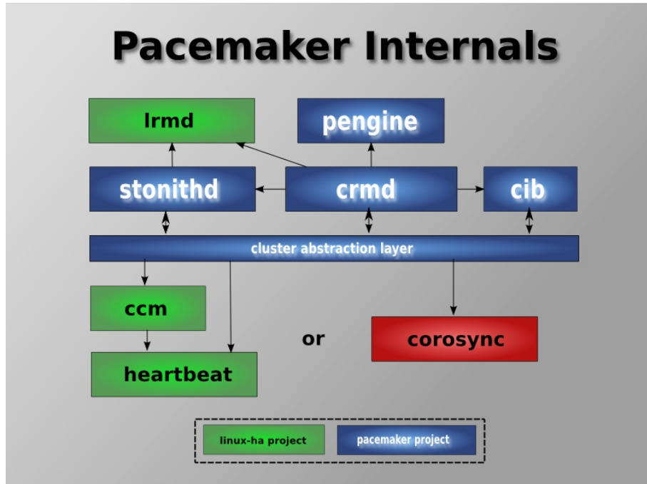
Figure 1.3. Internal Components
